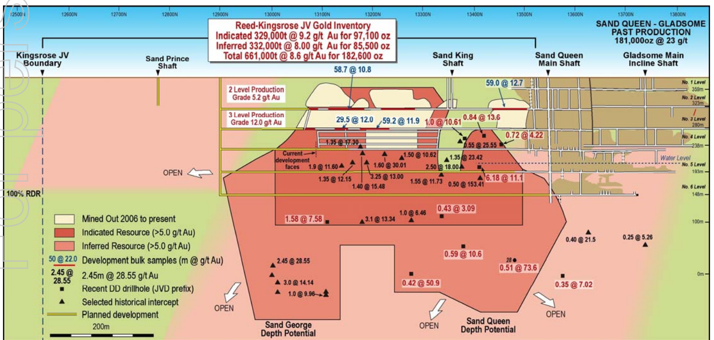
Figure 2 Vertical longitudinal projection of the Sand Queen Gold Mine, showing the resource outline in relation to current and planned development.
